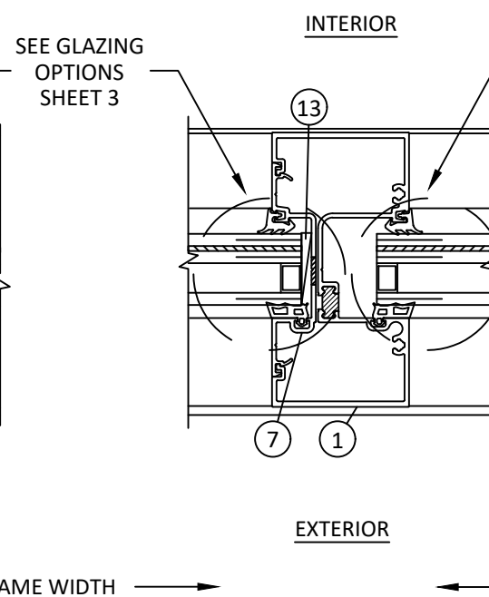
G 10 HORIZONTAL SECTION VERTICAL MULLION STANDARD CONFIGURATION
