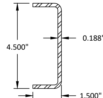
25 DOOR MULLION REINFORCEMENT
