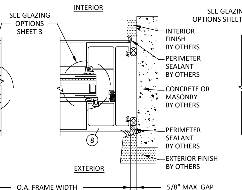
L 10 HORIZONTAL SECTION JAMB - DIRECT TO CONCRETE/MASONRY HEAVY CONFIGURATION
