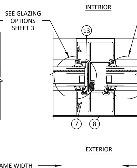
K 10 HORIZONTAL SECTION VERTICAL MULLION HEAVY CONFIGURATION
