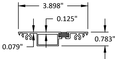
5 ANCHOR FILLER
