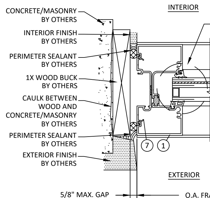
J 10 HORIZONTAL SECTION JAMB - CONCRETE/MASONRY W/ 1X BUCK HEAVY CONFIGURATION
