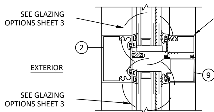
B 9 VERTICAL SECTION HORIZONTAL MEMBER
