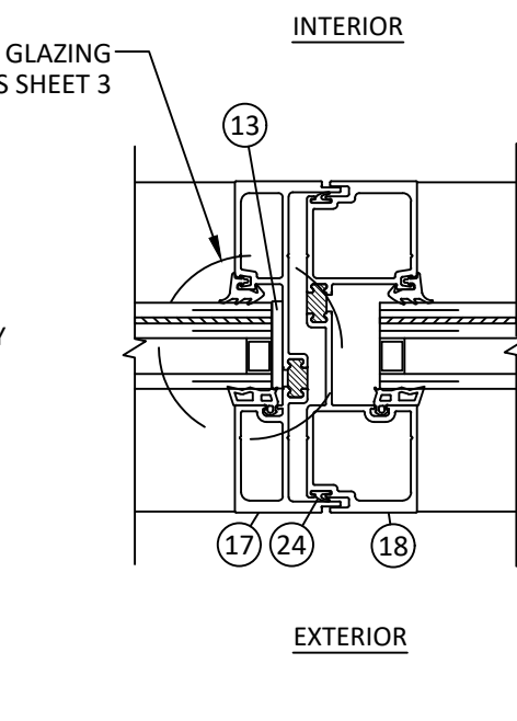
I 10 HORIZONTAL SECTION VERTICAL EXPANSION MULLION
