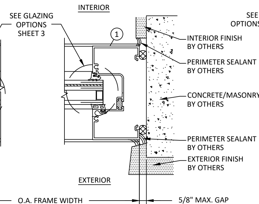
H 10 HORIZONTAL SECTION JAMB - DIRECT TO CONCRETE/MASONRY STANDARD CONFIGURATION
