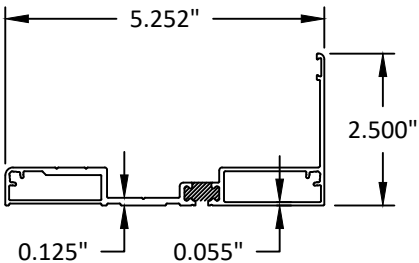
6 SILL FLASHING
