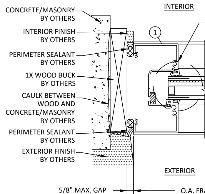
F 10 HORIZONTAL SECTION JAMB - CONCRETE/MASONRY W/ 1X BUCK STANDARD CONFIGURATION
