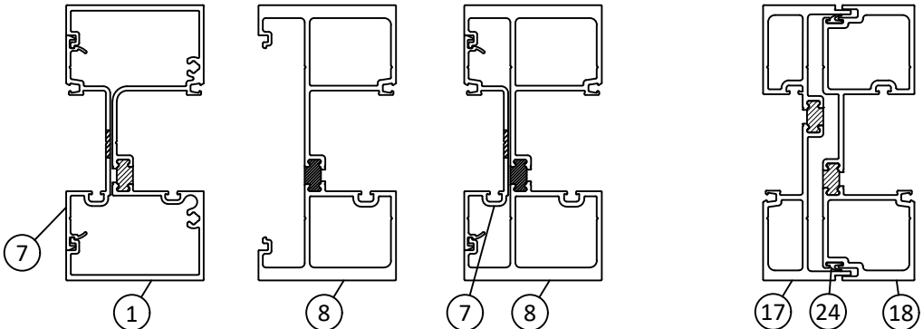
EXPANSION MULLION
